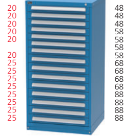
SEP3014AL 15 Drawers 336 Compartments Usable Drawer Heights 2-1/4 in. (57 mm) 3 in. (76 mm) 711 lbs. (323 kg.) Shipping Weight
