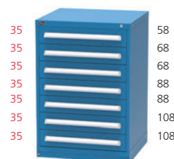
SEP2041AL 7 Drawers 120 Compartments Usable Drawer Height 4-5/8 in. (117 mm) 417 lbs. (189 kg.) Shipping Weight
